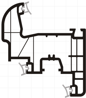
Sash 3D 7500 8ROL 8004
