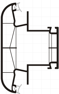
Mullion 3D 7500 8ROL 8008
