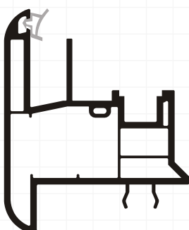
Mobile Mullion 3D 7500 8ROL 8012
